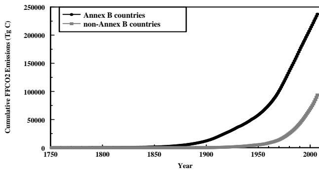
Fig. 3g. Cumulative FFCO 2 emissions for years 1751 to 2007, disaggregated by Kyoto Protocol status. Similar to Fig. 3c. This figure was created from summing the data in Fig. 3e. Data from Boden et al. (2010).
