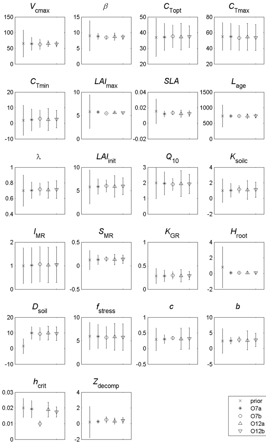
Figure 4. Resulting parameter values and their standard deviations. Prior values (crosses) are compared with optimized values: O7a (asterisks), O7b (open circles), O12a (open triangles), and O12b (open inverted triangles). Details on the optimized parameters can be found in Table 2. For the O12 scenarios: V_{cmax} , SLA , b , and c values represent means of the achieved monthly values with their standard deviations.
