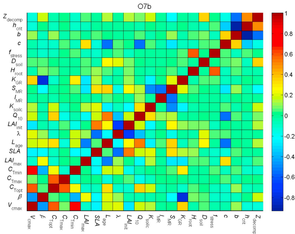
Figure 5. Posterior error correlation matrix after optimization O7b, assimilating both NEE and LE with scaled errors for NEE.
