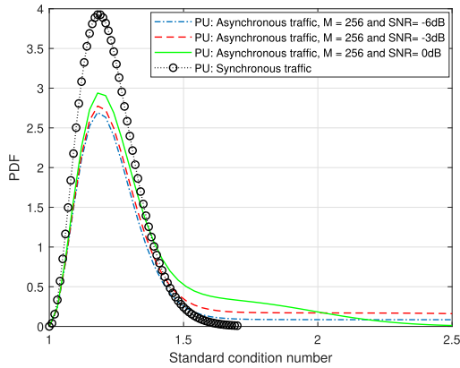
FIGURE 4. PDF under \mathcal{H}_0 of the SCN for different values of the SNR and N = 128 number of samples.
