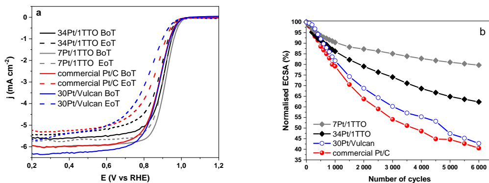
Figure 8. ORR polarization curves recorded at 1,600 rpm in O 2 saturated 0.1 M HClO 4 , at a scan rate of 20 mV s -1 (a) and ECSA variation (measured in N 2 saturated 0.1 M HClO 4 , at a scan rate of 20 mV s -1 ) upon electrochemical cycling up to 1.6 V vs RHE (b) for Pt nanoparticles deposited on 1Ta:SnO 2 (34 wt % Pt in black, 7 wt% in grey) and Vulcan (in blue) and for commercial Pt/C electrocatalyst (in red). The linear sweep voltammograms were recorded at the beginning and end of the accelerated stress test (BoT, full lines, and EoT, dotted lines).
