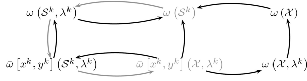
Fig. 3: Relationships of the optimal values involved in Algorithm 2.
