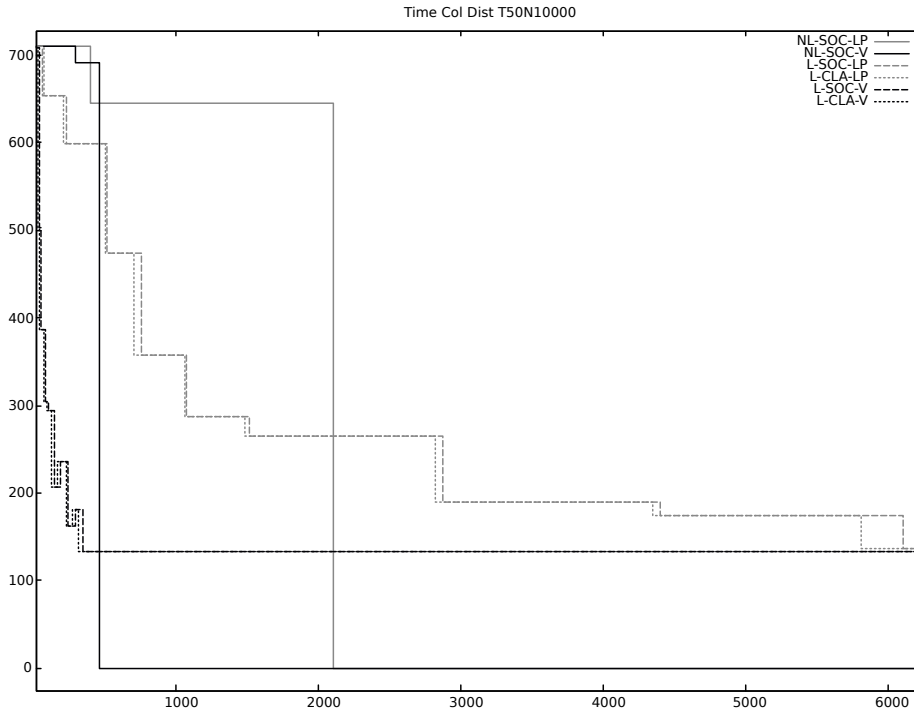
Fig. 6: Column distance to \mathcal{S} Vs. Time for T = 50 , N = 10.000 .
