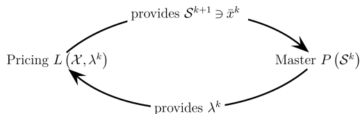
Fig. 1: CG feedback: (\bar{x}^k, \bar{y}^k) is optimal for L(\mathcal{X}, \lambda^k) , \lambda^k is dual-optimal for P(\mathcal{S}^k) .
