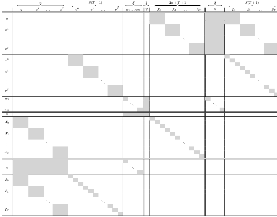
Fig. 10: Sparsity pattern of the Newton step for P with numerical enhancement.
