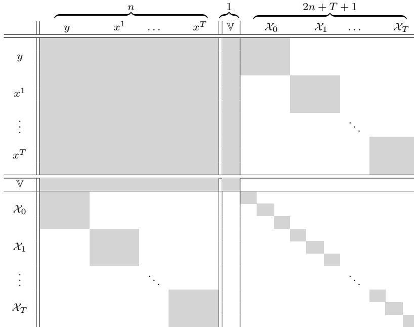
Fig. 9: Sparsity pattern of the Newton step for P without numerical enhancement.
