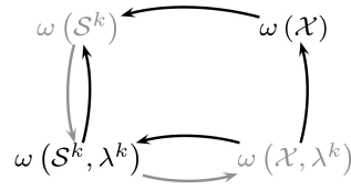
Fig. 2: Relationships of the optimal values involved in Algorithm 1.
