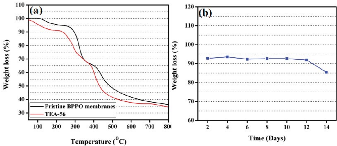
Fig. 8. (a) Thermogravimetric analysis of the pristine membrane and the membrane prepared with 56% triethanolamine (TEA-56) and (b) Weight loss of the TEA-56 membrane after immersion in HCl/FeCl 2 feed solution for two weeks at 55°C, showing high chemical stability.
