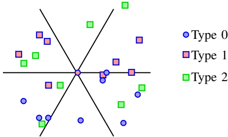
Fig. 3: Illustration of the distribution of the minutiae types (as defined in [1]) around a given minutia (red disk) for a sector decomposition into six sectors of equal angular ( 60^\circ )
