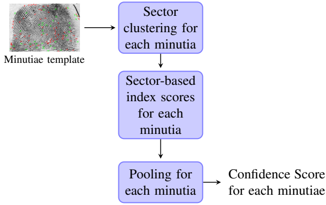
Fig. 2: Overall synopsis of the minutiae confidence index scoring.
