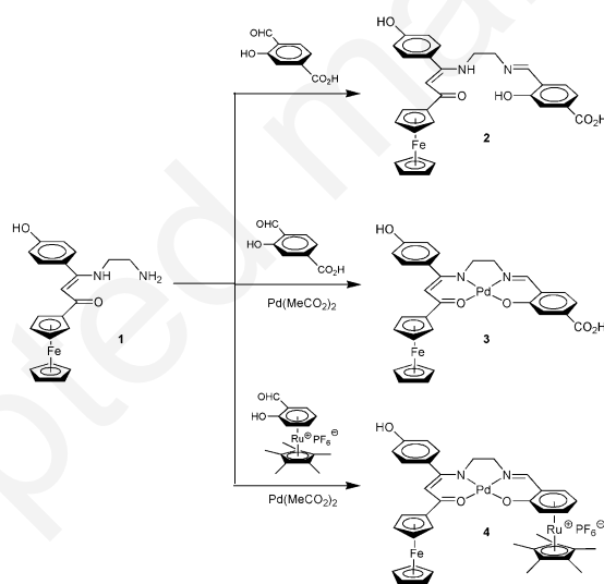
Scheme 1 Synthesis of the asymmetric Schiff base compounds 2-4 . All reactions are carried out in refluxing ethanol for 2 h.
