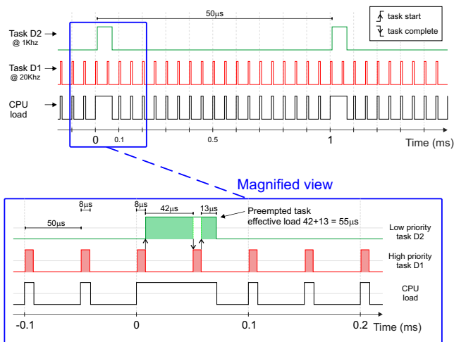
Fig. 8. Scope measurement of task execution for a Multi-rate model with a multi-tasking rate monotonic scheduler
