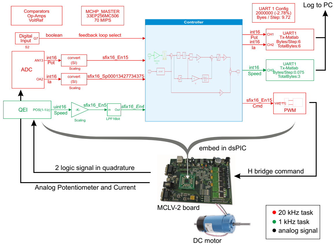
Fig. 7. Control global scheme example. The model is compiled and run as a standalone program on the targeted board
