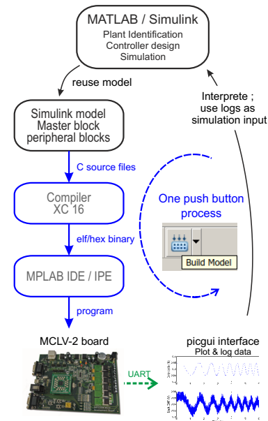
Fig. 6. Rapid Prototyping Scheme
