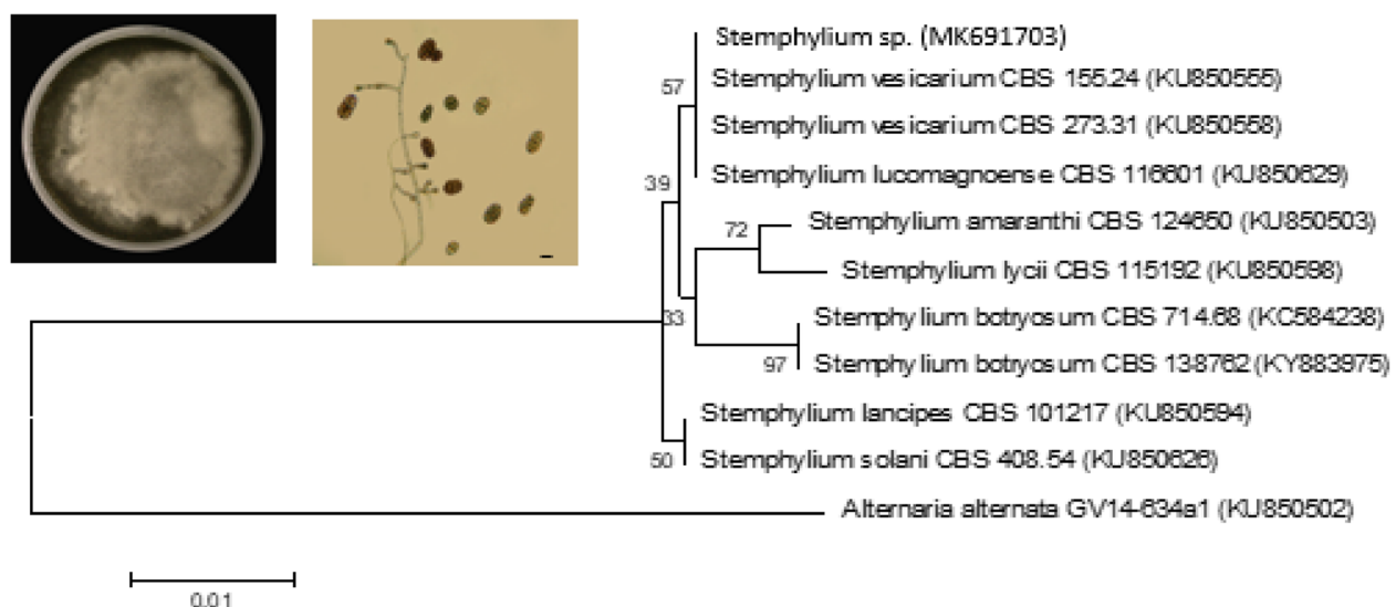
Fig. 1 Phylogenetic reconstruction for the strain Stemphylium sp., based on ITS analysis [17] using the neighbor-joining algorithm (NJ) method and 1000 replicate bootstraps. ITS sequences were deposited in the NCBI under accession number MK691703. Culture plate of Stemphylium sp. and conidiophores and conidia (scale bar = 10 µm)
