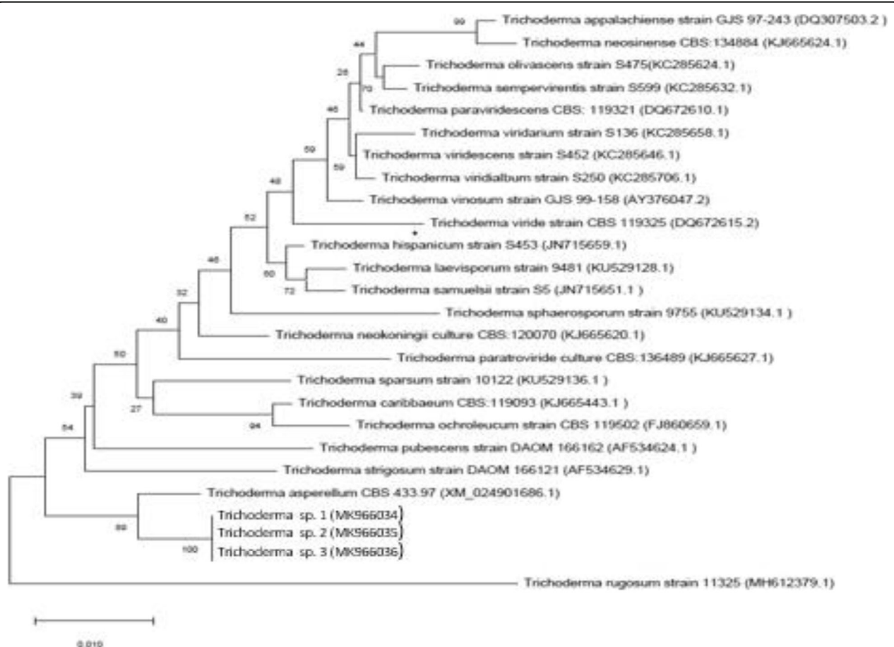
Fig. 3 Phylogenetic reconstruction for the strains Trichoderma sp. 1, 2 and 3 based on elongation factor 1-alpha (EF1a) analysis using the neighbor-joining algorithm (NJ) method and 1000 replicate bootstraps (MK966034, MK966035 and MK966036 are the accession numbers of Trichoderma 1, 2 and 3 respectively)
