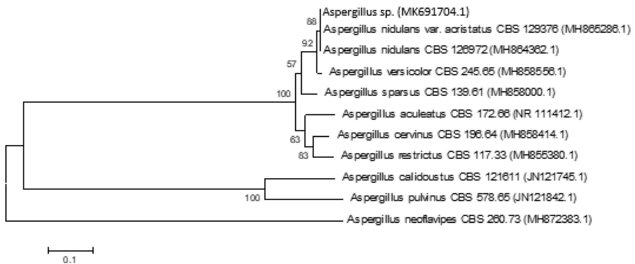
Fig. 2 Phylogenetic reconstruction for the strain Aspergillus sp., based on ITS analysis using the neighbor-joining algorithm (NJ) method and 1000 replicate bootstraps, ITS sequences were deposited in the NCBI under accession number MK691704
