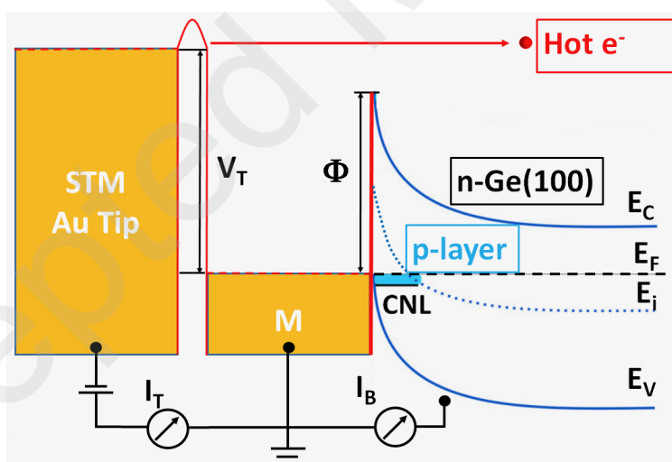
Figure 1: Upper panel: Schematic diagram of the metal/Ge(100) junctions and the experimental setup for BEEM measurements, I_B(V) , acquired under dark at 80 K. I_T(V) corresponds to the injected current of tunneling electrons. Lower panel: Schematic diagram for energy bands at the junction.
