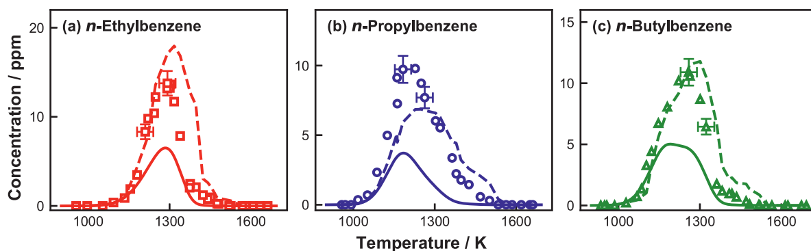
Fig. 13. Bibenzyl ( C_6H_5C_2H_4C_6H_5 ) concentrations as a function of T_5 in the pyrolysis of C_8 – C_{10} linear alkylbenzenes. Symbols: measurements; Solid lines, simulations with constant pressure of 20 bar and reaction time of 4.0 ms. Dashed lines, simulations with measured pressure profiles up to 10.0 ms.
