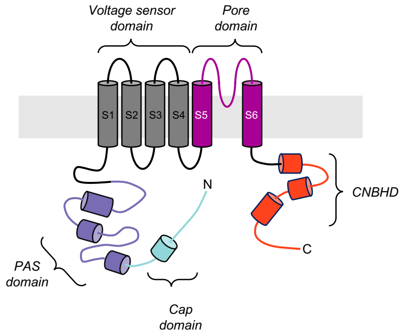
Figure 1. Schematic of the hERG3 channel subunit. hERG, which is part of the EAG family of ion channels, has four subunits which assemble to form a tetrameric structure (left). Each subunit contains a transmembrane region as well as cytoplasmic N- and C-terminal regions. The transmembrane region contains voltage sensor (helices S1-S4, dark grey) and pore-forming (helices S5-S6, magenta) domains inside the membrane bilayer. The C-terminal cytoplasmic region contains a cyclic nucleotide-binding homology domain (CNBHD, red), which is connected to the transmembrane region via a structured domain usually referred to as the C-linker. The N-terminal cytoplasmic region (approximately 400 residues) contains a region that is known as the eag domain (residues 1-135), which itself comprises a Cap domain (residues 1-25, light blue) and a PAS domain (residues 26-135, purple). This eag-domain fragment (residues 1-135) has been expressed in this work and is referred to as hERG3-eag in this paper.
