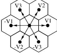
Fig. 6. Connectivity on the hexagonal grid. Filled circles represent grid points, hexagons represent pixels. Vectors \mathbf{V}_1 , \mathbf{V}_2 , \mathbf{V}_3 , and their negatives relate each grid point to its neighbors.
