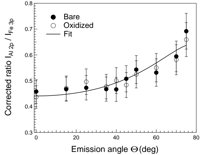
FIG. 4. Comparison of angular variation of the corrected ratio I_{\text{Al}2p}^c/I_{\text{Fe}3p}^c for the metallic components on the bare (filled circles) and oxidized (open circles) \text{Fe}_{0.85}\text{Al}_{0.15} (110) surface. The chosen error bars of 10 % on the experimental ratio match with data dispersion. The continuous line corresponds to a fit with a continuous profile of segregation (see text).
