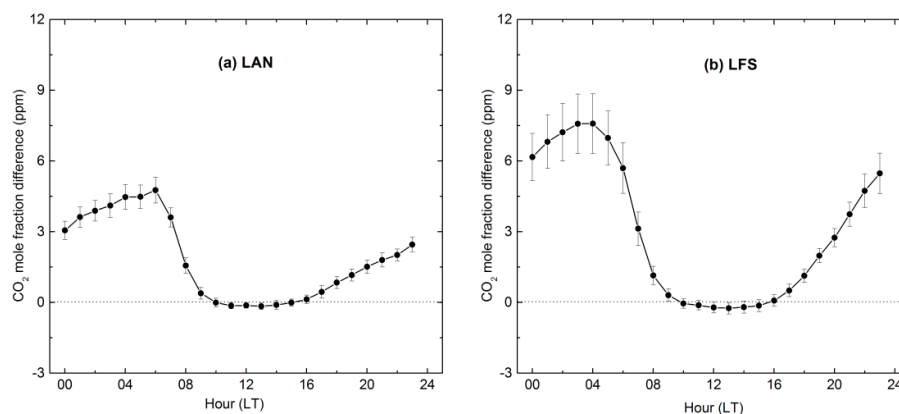
Fig. 4. Diurnal differences of hourly CO 2 mole fractions between 10 m and the top of each tower at the two regional stations. (a) LAN station, CO 2 concentration at 10 m minus 50 m. (b) LFS station, 10 m minus 80 m. Error bars indicate confidence intervals of 95 %.
