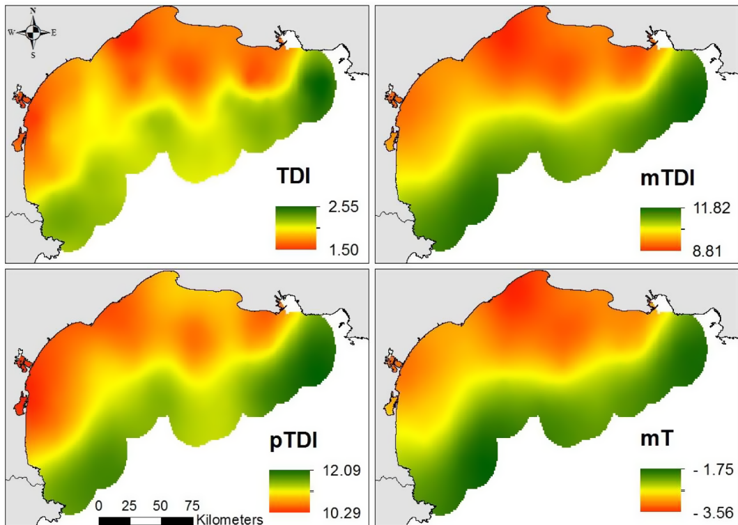
Fig. 6. Distribution pattern of benthic sensitivity to trawling in the Gulf of Lion (MEDITS data).
