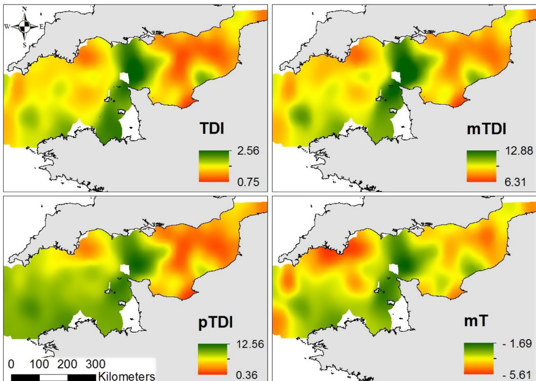
Fig. 8. Distribution pattern of benthic sensitivity to trawling in the English Channel (CGFS and CAMANOC data).
