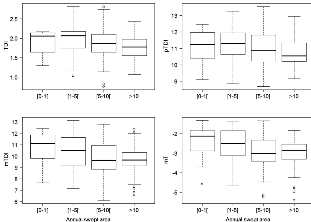
Fig. 2. Values of the four selected indices by class of abrasion in the Gulf of Lion.
