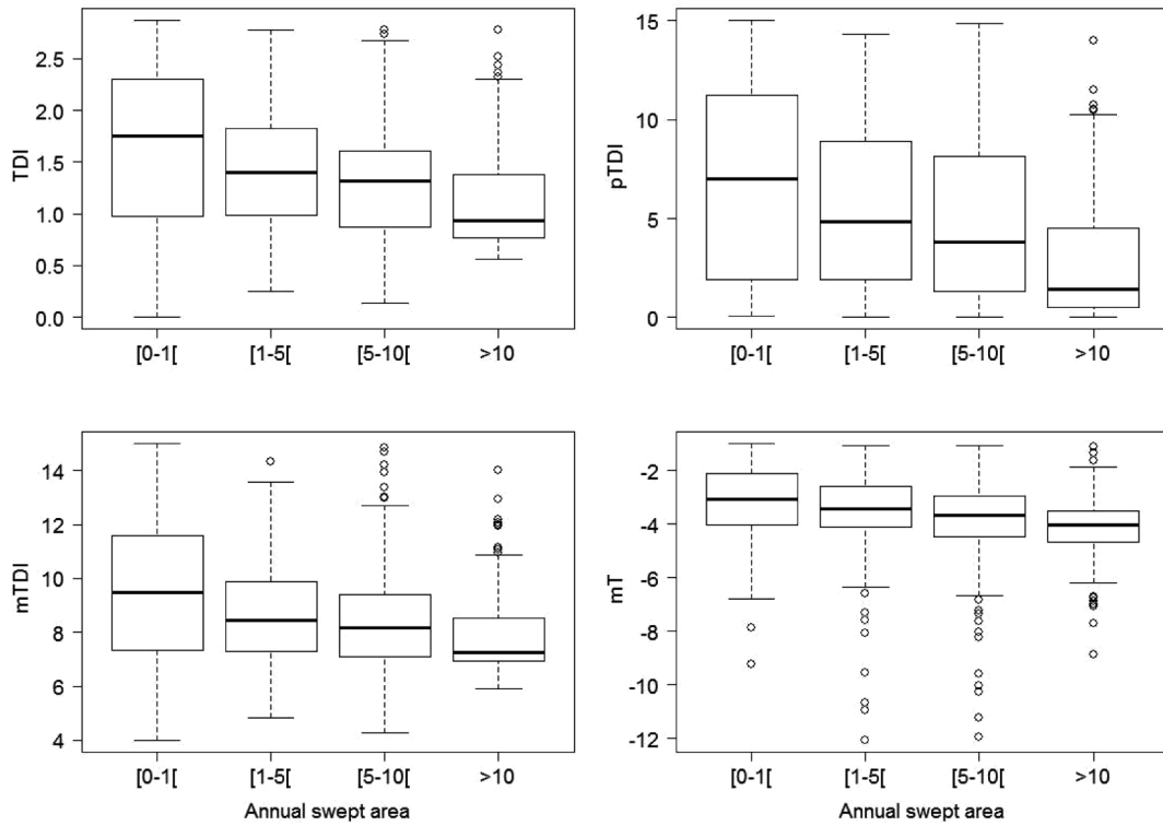
Fig. 5. Values of the four selected indices by class of abrasion for the CGFS and CAMANOC data (English Channel).
