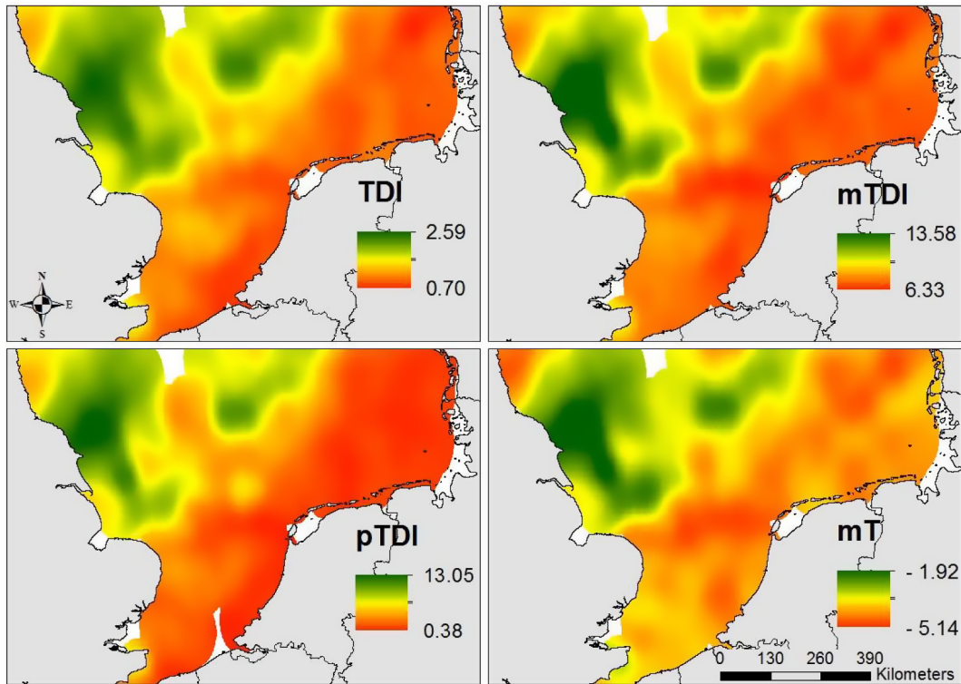
Fig. 7. Distribution pattern of benthic sensitivity to trawling in the southern North Sea (IBTS data).
