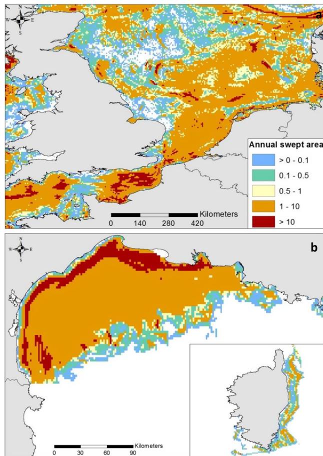
Fig. 1. 90th inter-annual percentile of the abrasion in the English Channel and southern North Sea during the period 2009–2017 (a) and in the Gulf of Lion during the period 2009–2017 (b).
