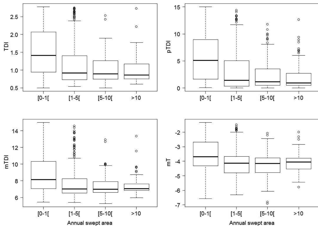
Fig. 4. Values of the four selected indices by class of abrasion for the IBTS data (eastern English Channel and southern North Sea).
