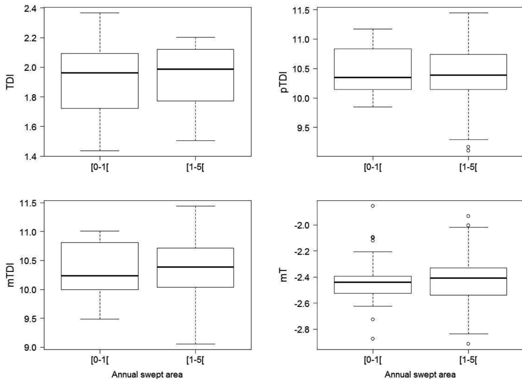
Fig. 3. Values of the four selected indices by class of abrasion in Corsica.
