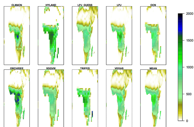
Fig. 4. Average net primary productivity (NPP) for each DGVM and model mean over the period 1990–2009, units, \text{g C m}^{-2} \text{ yr}^{-1} (from Sitch et al., 2014).
