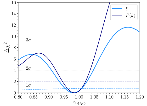
Figure 16. The BAO likelihood obtained from the combination of NGC and SGC results. We display our results ( \xi ) and also the Fourier-space ( P(k) ) results from de Mattia et al. (2020). The dashed curves show the results for the model with no BAO.
