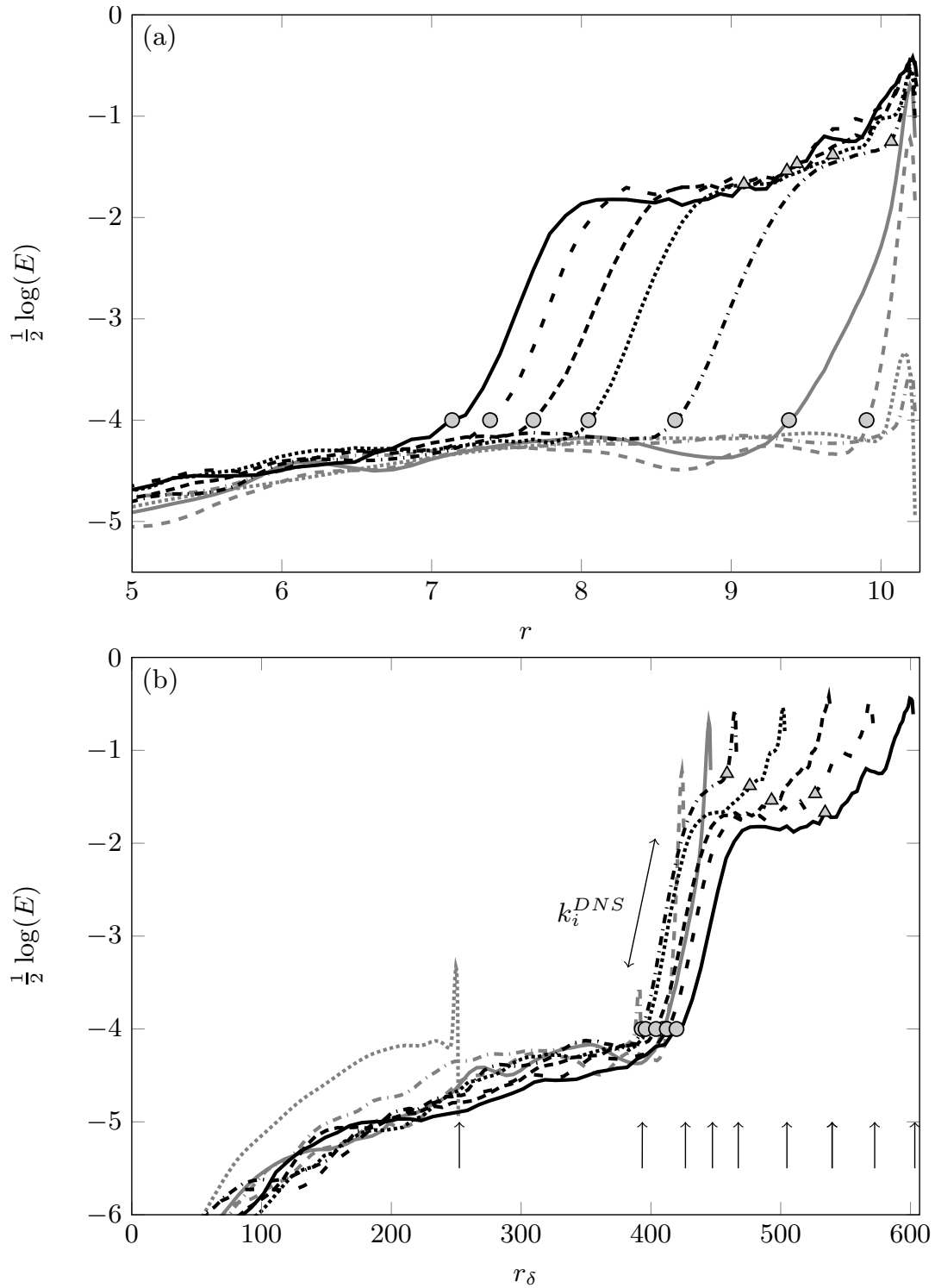
Figure 6. (Color online) Radial profiles of the turbulent kinetic energy E in the rotor boundary layer at z = 0.97 , and for various global Reynolds numbers: \cdots Re = 0.7 \times 10^5 ; -\cdot-\cdot- Re = 1.7 \times 10^5 ; --- Re = 2 \times 10^5 ; — Re = 2.2 \times 10^5 ; -\cdot-\cdot- Re = 2.4 \times 10^5 ; \cdots Re = 2.8 \times 10^5 ; -\cdot-\cdot- Re = 3.2 \times 10^5 ; --- Re = 3.6 \times 10^5 and — Re = 4 \times 10^5 . The symbols represent the locations of the primary ( \circ ) and the secondary fronts ( \triangle ) as defined in figure 4. The arrows in (b) indicate the edge local Reynolds number r_{\delta_{edge}} (maximum value of r_\delta ) for each Re .
