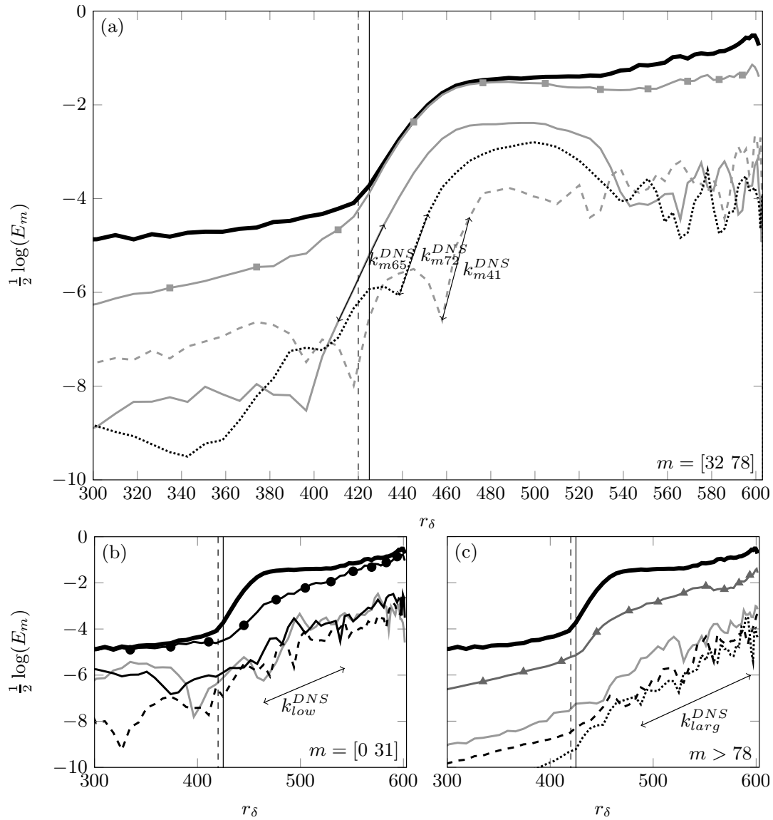
Figure 7. Kinetic energies of the perturbation for some selected azimuthal wavenumbers m in the ranges of (a) intermediate m \in [32, 78] : m = 41 ---, m = 65 — and m = 72 \cdots (b) low m = [0, 31] : m = 0 —, m = 10 — and m = 30 ---, (c) large m > 78 : m = 90 —, m = 118 --- and m = 140 \cdots at Re = 4 \times 10^5 . The thick black lines show the total energy ( 1/2 \log(E) ) shown in figure 6 and lines with symbols show the total energy restricted to each range. The vertical solid line indicates the absolute instability transition r_{\delta_{c/a}} = 425 of the mean flow and dashed line represents the primary front of DNS defined in figure 4. The spatial growth rates are estimated as k_{i,m41}^{DNS} = -0.18 , k_{i,m65}^{DNS} = -0.1 , k_{i,m72}^{DNS} = -0.13 and for low and large m , the spatial growth rates are approximately estimated as k_{i,low}^{DNS} \simeq -0.014 and k_{i,larg}^{DNS} \simeq -0.019 .
