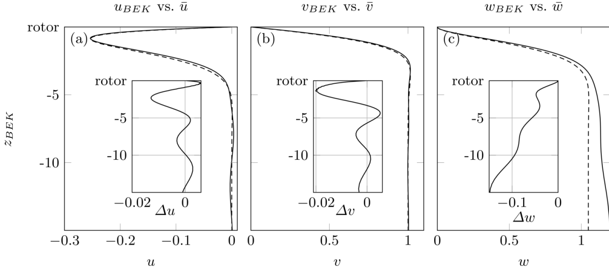
Figure 2. Comparisons of the velocities near the rotor between the mean flow solution — at r = 7.2 and Re = 4 \times 10^5 , and the BEK self-similarity solution - - for Ro = -0.72 (mean Ro of the mean flow): (a) radial velocity u_{BEK} and \bar{u} (b) azimuthal velocity v_{BEK} and \bar{v} , and (c) axial velocity w_{BEK} and \bar{w} . The inserted plots show the differences \Delta \mathbf{u} = \mathbf{u}_{BEK} - \bar{\mathbf{u}} . Here, the length and velocities are scaled as in Lingwood (1997), i.e. \delta, r^* \Omega^* Ro for u and v and \Omega^* Ro for w , where the superscript * indicates dimensional values, and \Omega^* and Ro are defined in equation (1).
