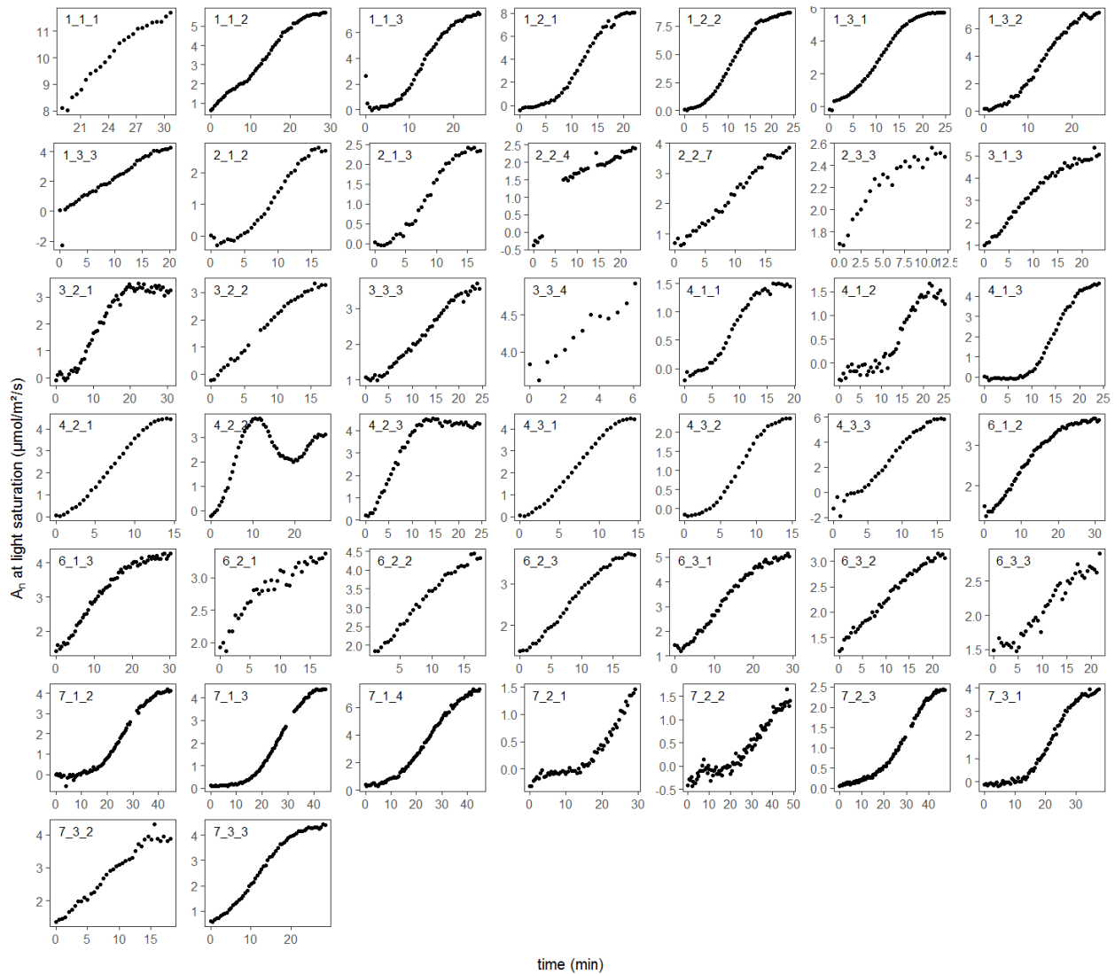
Fig. S3 Actual data of continuously measured leaf net photosynthetic rate ( A_n ; \mu\text{mol/m}^2/\text{s} ) at light saturation after excision and transport of the branch. Time 0 corresponds to the placement of the leaf in the gas exchange chamber. The ID number of each plot refers to the tree number (1-7; no data available for tree 5 since we did not log A_n continuously), followed by the canopy height (1 = upper canopy, 2 = middle canopy, 3 = lower canopy) and the number of the replicate.
