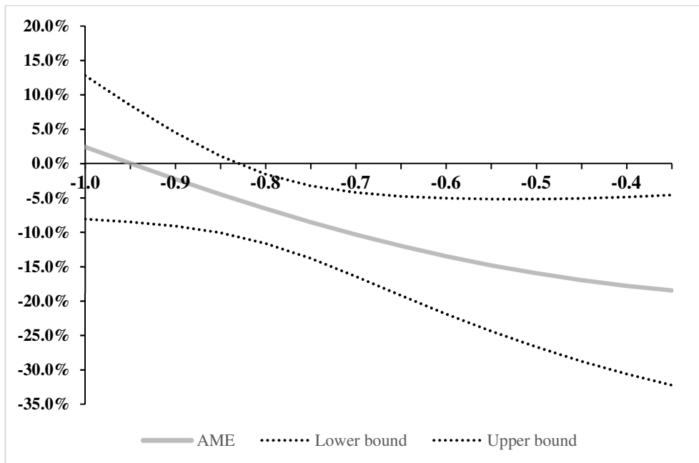
Figure 1: AME of the local deals for different levels of corruption and a 95% confidence interval
