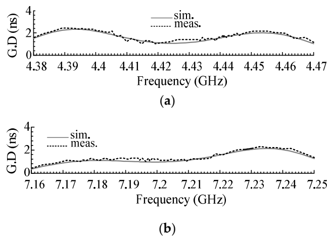
Figure 14. Group delay (GD): (a) first passband, (b) second passband.
