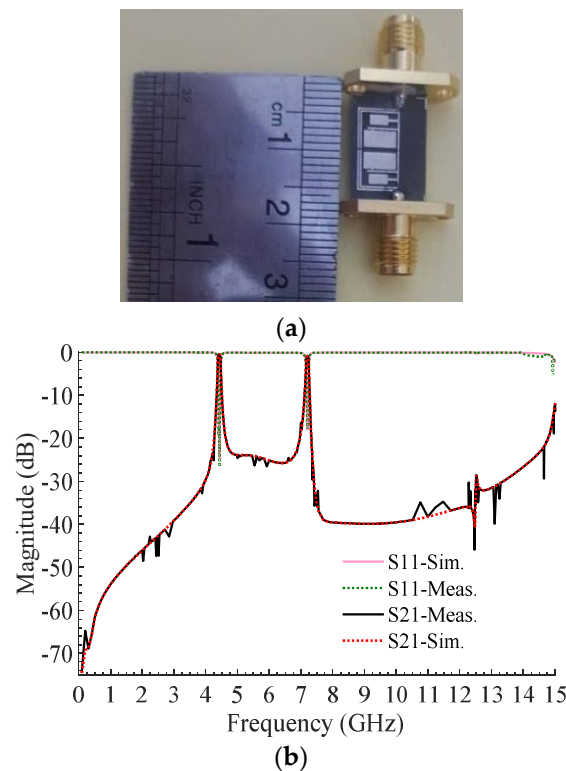
Figure 13. Proposed BPF: (a) A photo of the fabricated filter; (b) Simulation and measurement results.
