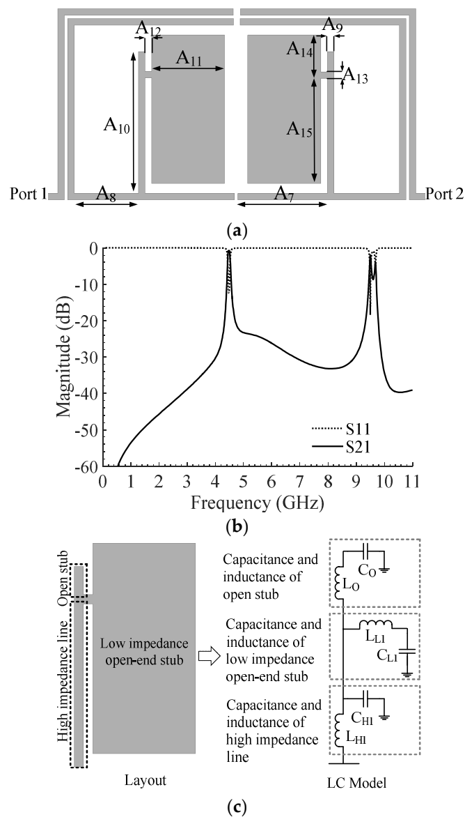
Figure 5. Integration of flag-shaped resonators with the bended coupled system. (a) Layout, (b) EM simulation, (c) LC model of flag-shaped resonator. The dimensions of the introduced flag-shaped resonators are as follows: A_7 = 2.7 , A_8 = 1.9 , A_9 = 0.2 , A_{10} = 4.3 , A_{11} = 2.2 , A_{12} = 0.2 , A_{13} = 0.2 , A_{14} = 1.32 , A_{15} = 3.2 (all in mm).
