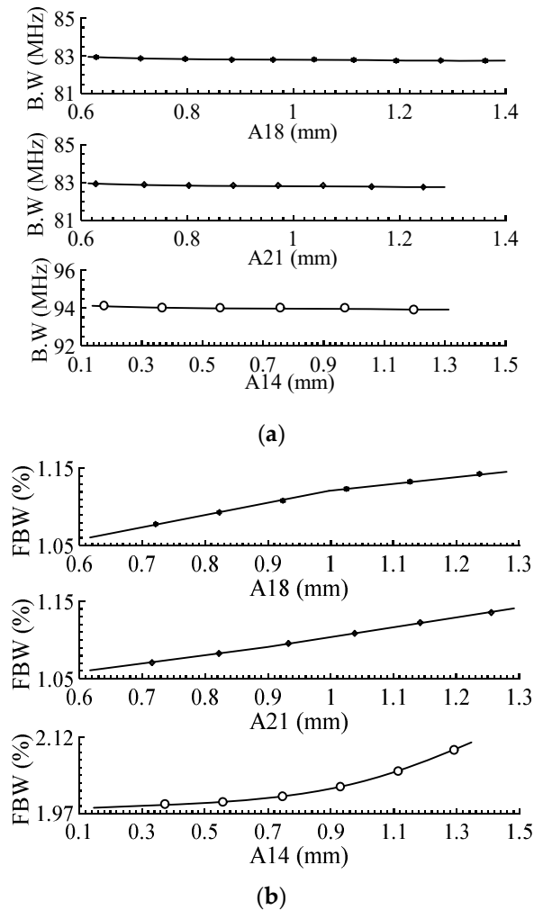
Figure 11. (a) Variations of bandwidth as a function of A_{18} , A_{21} and A_{14} , (b) Variations of fractional bandwidth (FBW) as a function of A_{18} , A_{21} and A_{14} .
