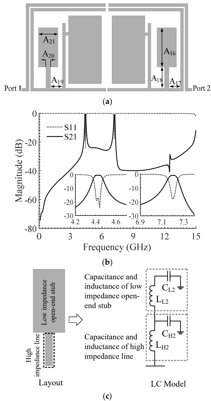
Figure 6. Completed dual-band bandpass filter (BPF): (a) Layout, A_{16} = 2.6 , A_{17} = 0.8 , A_{18} = 1.4 , A_{19} = 0.8 , A_{20} = 0.3 , A_{21} = 1.3 (all in mm), (b) EM simulation, (c) LC model of stepped-impedance resonator.
