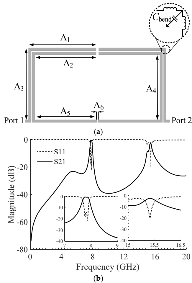
Figure 2. Bended coupling system: (a) Layout, A_1 = 5.3 , A_2 = 4.8 , A_3 = 5.6 , A_4 = 5.1 , A_5 = 4.8 , A_6 = 0.1 (all in mm), (b) EM simulation.
