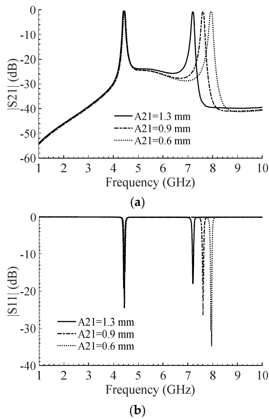
Figure 9. Adjustability of the upper band of the proposed BPF by varying A_{21} : (a) |S_{21}| , (b) |S_{11}| .
