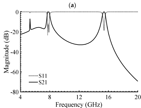
Figure 3. Bended coupling system: (a) lumped-element circuit (LC) model, (b) LC simulation.
