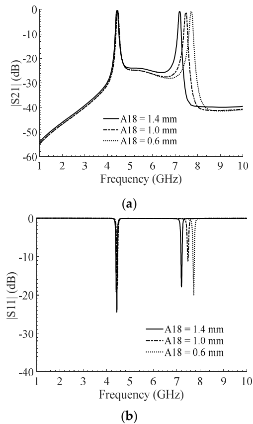
Figure 10. Adjustability of the upper band of the proposed BPF by varying A_{18} : (a) |S_{21}| , (b) |S_{11}| .
