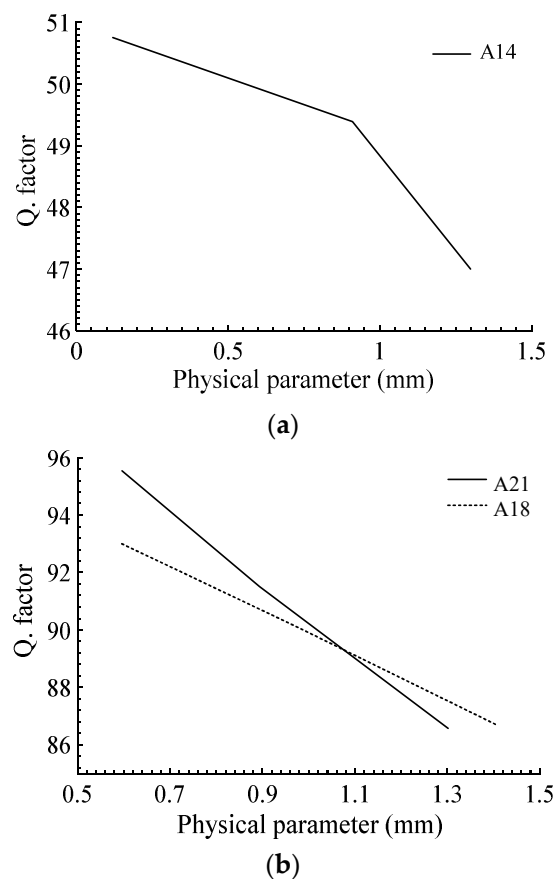
Figure 12. (a) Variations of Q. factor versus physical parameters: (a) A 14 , (b) A 18 and A 21 .
