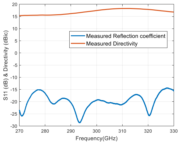
FIGURE 8. Measured reflection coefficient (S11), and directivity for the prototype of the 300 GHz CP horn antenna.
