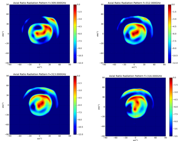
FIGURE 13. Measured normalized 2D axial ratio plots at 309 GHz, 312 GHz, 313 GHz, and 316 GHz.
