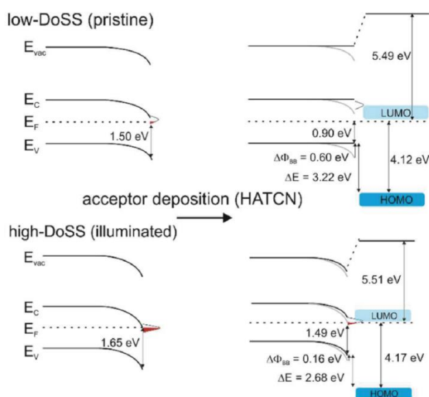
Figure 13. Interfacial energy level diagrams, derived from the PES data for pristine (low-DoSS) and defective (high-DoSS) MAPbI 3-x Cl x samples, without (left) and with (right) HAT-CN overlayer on top. Reproduced with permission. [196] Copyright 2017, American Chemical Society.
