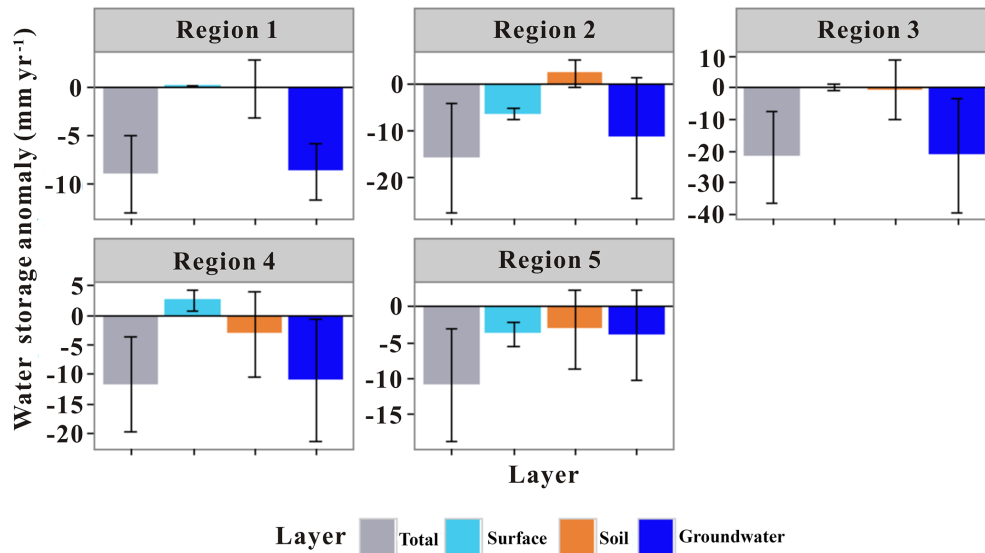
Figure 5. Contributions of different hydrological storages to TWS changes in five hotspots. Uncertainties represent 95 % confidence intervals.
