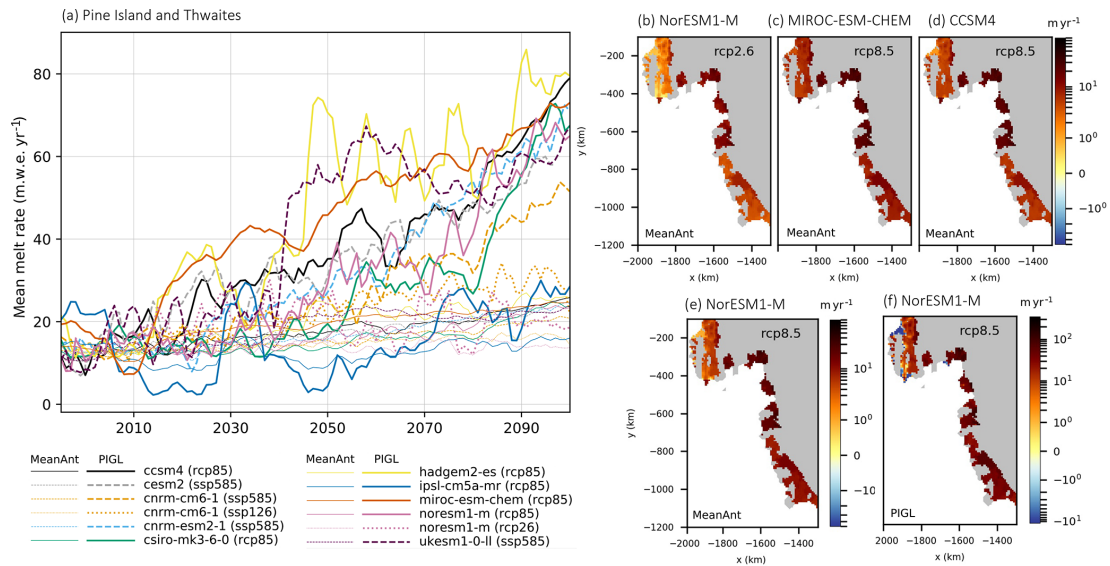
Figure 7. Mean cavity basal melt rates (m.w.e. yr -1 ) under the RCP2.6, RCP8.5, SSP1-2.6, and SSP5-8.5 scenarios over the 21st century for MeanAnt and PIGL calibrations and nonlocal parameterizations in the Amundsen Sea sector. (a) Time series for Pine Island and Thwaites ice shelves obtained with MeanAnt (thin lines) and PIGL (thick lines) calibrations (adapted from Jourdain et al., 2020). Spatial patterns of mean sub-shelf basal melt rate from 2081 to 2100 for the Tier 1 models assuming MeanAnt calibration for (b) NorESM1-M under RCP2.6, (c) MIROC-ESM-CHEM under RCP8.5, (d) CCSM4 under RCP8.5, and (e) NorESM1-M under RCP8.5 and PIGL calibration for (f) NorESM1-M under RCP8.5. The projections from the MeanAnt and PIGL calibrations assume that the ice shelf cavities have not evolved and are set to the present day.
