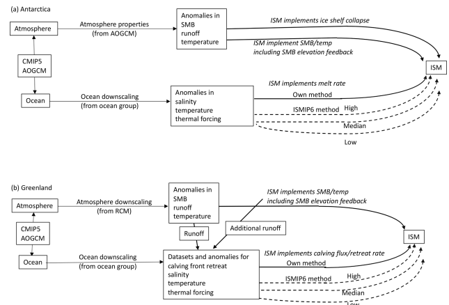
Figure 1. Overview of ISMIP6 (a) Antarctic and (b) Greenland projection framework, illustrating the strategy for translating the CMIP atmospheric and oceanic properties into climatic forcing for ice sheet models.
