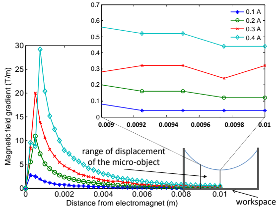
Fig. 3. Magnetic field gradient produced by one electromagnet along the (o, x) axis. Measurements are made using a teslameter (F.W Bell, Model 7010) based on the use of an Hall probe. The magnetic field gradient is considered constant further than 9 mm away from the electromagnet. Thus, it is constant along the trajectory of the micro-object.
