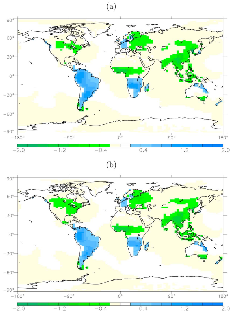
Figure 7. Flux increments (posterior minus prior fluxes) for the (a) first and (b) second weeks of 2000 (gC m -2 per day).
