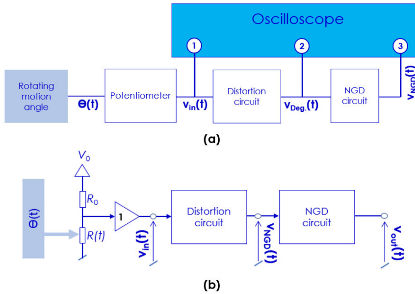
FIGURE 15. Illustration of (a) experimental setup and (b) sensor conditioning circuit.
