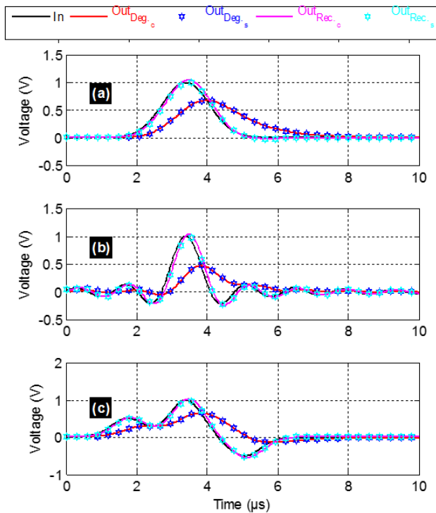
FIGURE 14. Comparison of simulated and calculated transient responses form the NGD reconstructed circuit shown in Fig. 6: (a) Gaussian, (b) sinc and (c) arbitrary waveform pulse signals.
