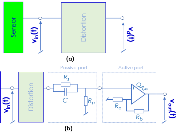
FIGURE 5. Diagram of (a) distorted and (a) reconstructed sensor with NGD circuit topology.
