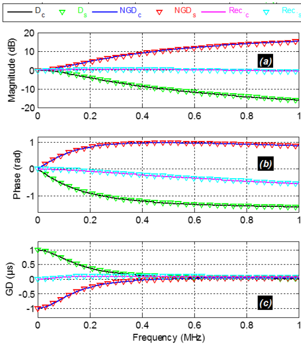
FIGURE 11. Comparison of simulated and calculated TF (a) magnitudes, (b) phases and (c) GDs of the reconstructed circuit POC shown in Fig. 6.
