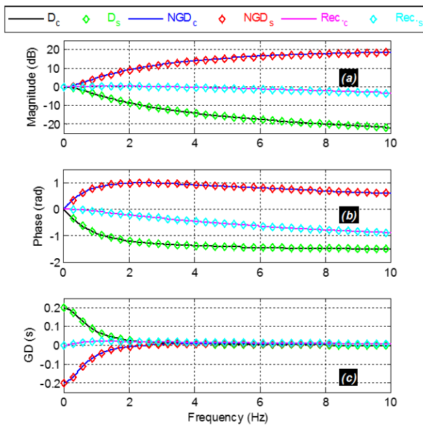
FIGURE 16. Comparison of simulated and calculated (a) magnitudes, (b) phases and (c) GDs.
