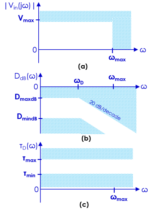
FIGURE 4. Specifications: (a) input signal amplitude, (b) distortion magnitude and (c) group delay.
