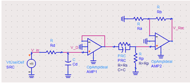
FIGURE 6. Design of POC including the distortion R_d C_d -circuit connected with the NGD circuit.
