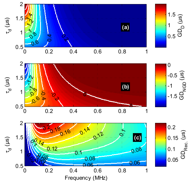
FIGURE 9. Cartographies of (a) distorted (“D”), (b) NGD and (c) reconstructed (“Rec.”) calculated TF GDs versus \tau_d and frequency.
