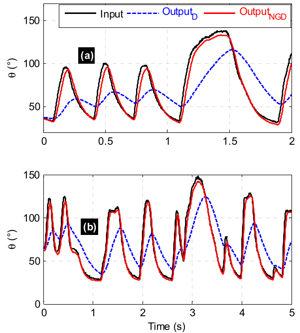
FIGURE 17. Comparison of distorted and reconstructed measured transient signals form the experimental setup shown in Fig. 15 with: (a) 2 s and (b) 5 s time durations.
