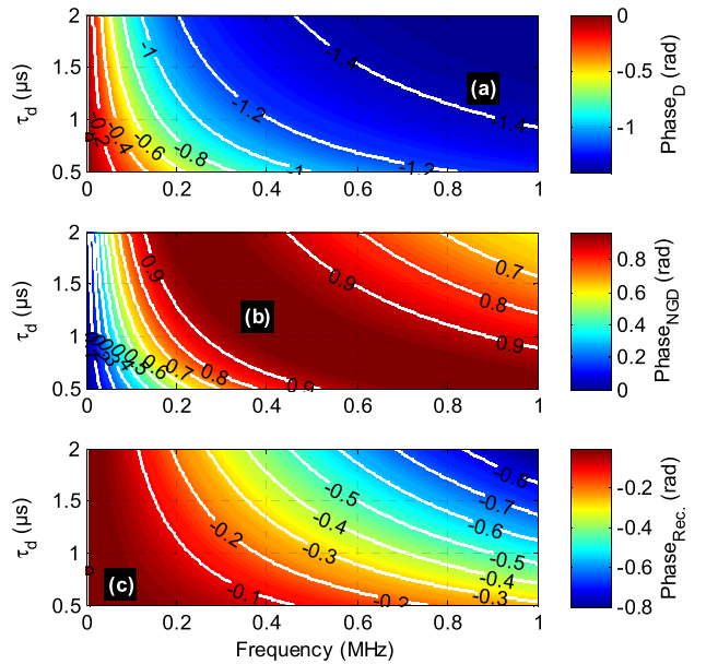
FIGURE 8. Cartographies of (a) distorted (“D”), (b) NGD and (c) reconstructed (“Rec.”) calculated TF phases versus \tau_d and frequency.
