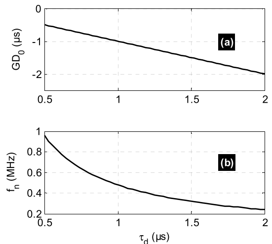
FIGURE 10. (a) GD value and (b) NGD cut-off frequency corresponding to the NGD TF GD cartography shown in Fig. 7.
