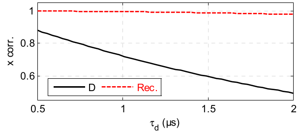
FIGURE 13. Comparison of cross correlations between the distorted (“black solid line”) vs reconstructed (“red dashed line”) and sensed signals.
