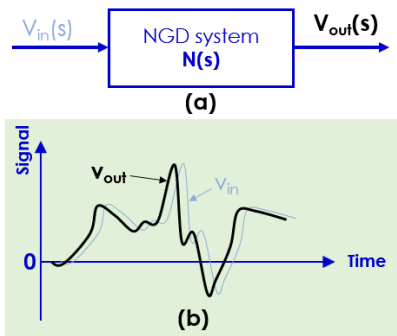
FIGURE 1. (a) NGD system black box and (b) typical transient response of NGD system [28]–[32].
