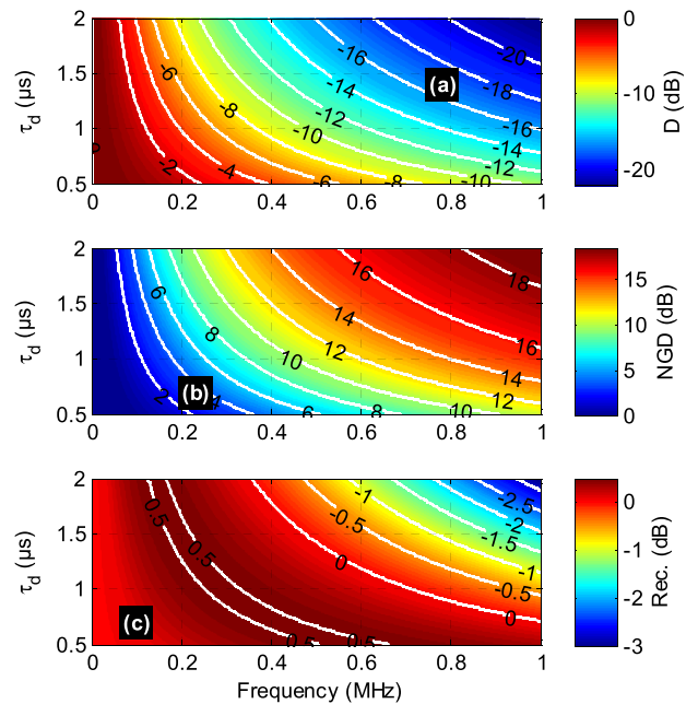
FIGURE 7. Cartographies of (a) distorted (“D”), (b) NGD and (c) reconstructed (“Rec.”) calculated TF magnitudes versus \tau_d and frequency.
