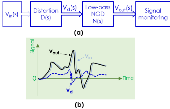
FIGURE 3. (a) Classical and (b) reconstructed sensor signal monitoring synoptic diagram.
