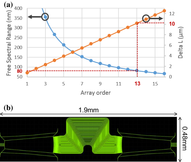
Figure 1: (a) Graphic showing dependence between FSR, array order and array waveguide length difference, (b) AWG layout.
