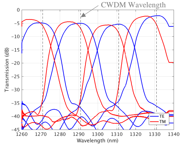
Figure 3: AWG experimental spectral response for TE and TM polarisation. (Characterisation by edge coupling.)
