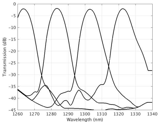
Figure 2: Standard AWG experimental spectral response for TM polarisation. (Characterisation by grating coupler.)
