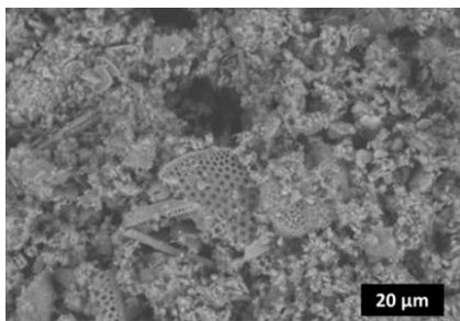
Fig. 2 SEM image of Hranfa's marl
