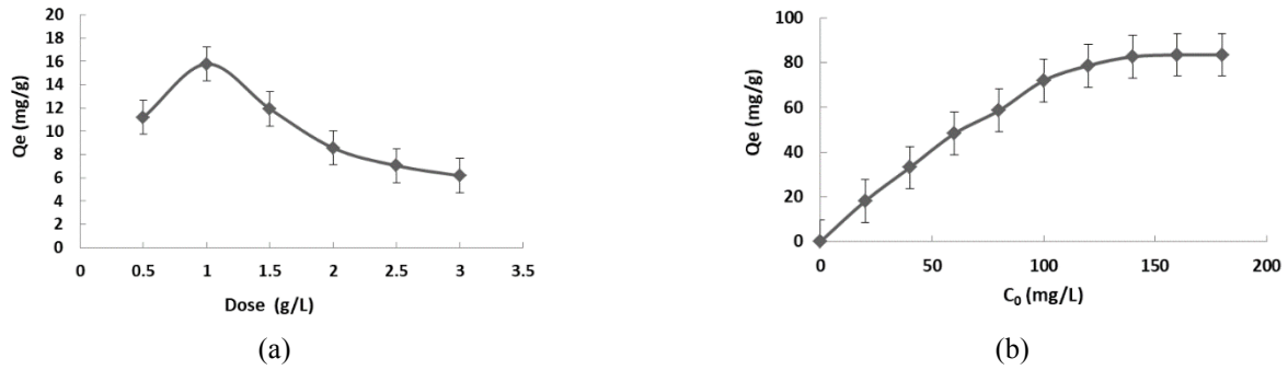
Fig. 5 Adsorption results in batch conditions for pH = 6 and T = 20 ± 2 °C. (a) Evolution of the adsorption capacity Q_e as a function of the adsorbent dose. C_0 was equal to 20 mg L -1 ; (b) Effect of the initial concentration of dye, C_0 , on the adsorption capacity Q_e . The dose was equal to 1 g L -1 .
