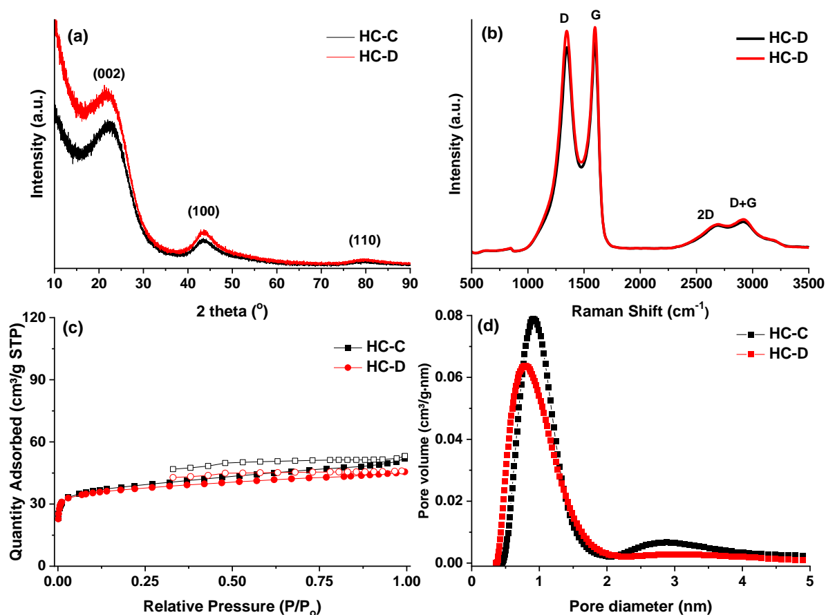
Figure 4. Characterization of the selected cellulose (black trace) and cotton (red trace)-based hard carbon SSEs: a) XRD spectra, b) Raman spectra, c) N 2 adsorption-desorption isotherms, and d) NLDFT pore size distribution.
