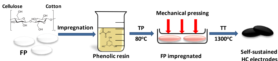
Scheme 1. Synthesis procedure used to prepare hard carbon (HC) SSEs using FPs impregnated with phenolic resin, thermopolymerized (TP) at 80°C and thermally treated (TT) at 1300°C.
