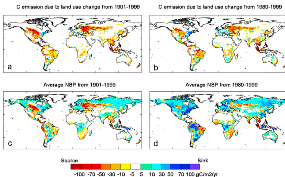
Figure 10. Spatial distribution of carbon emissions from land use change (simulation S6 – S5) and net carbon exchange (NBP) associated with all factors including climate, atmospheric CO 2 and land use (simulation S1 + S6 – S5) for the periods 1901–1999 and 1980–1999.
