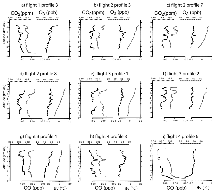
Fig. 6. Nine selected vertical profiles of the April 2006 campaign which are discussed in the text. The CO 2 profiles are in thick black to the left-hand side of each plot, CO in light grey, O 3 in black and potential temperature in dark grey to the right-hand side of each plot.
