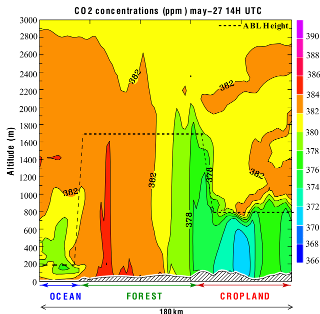
Figure 5. Vertical cross section of simulated CO 2 concentrations (ppm) on May-27 at 1400 UTC. The dotted line represents the approximate height of the atmospheric boundary layer.
