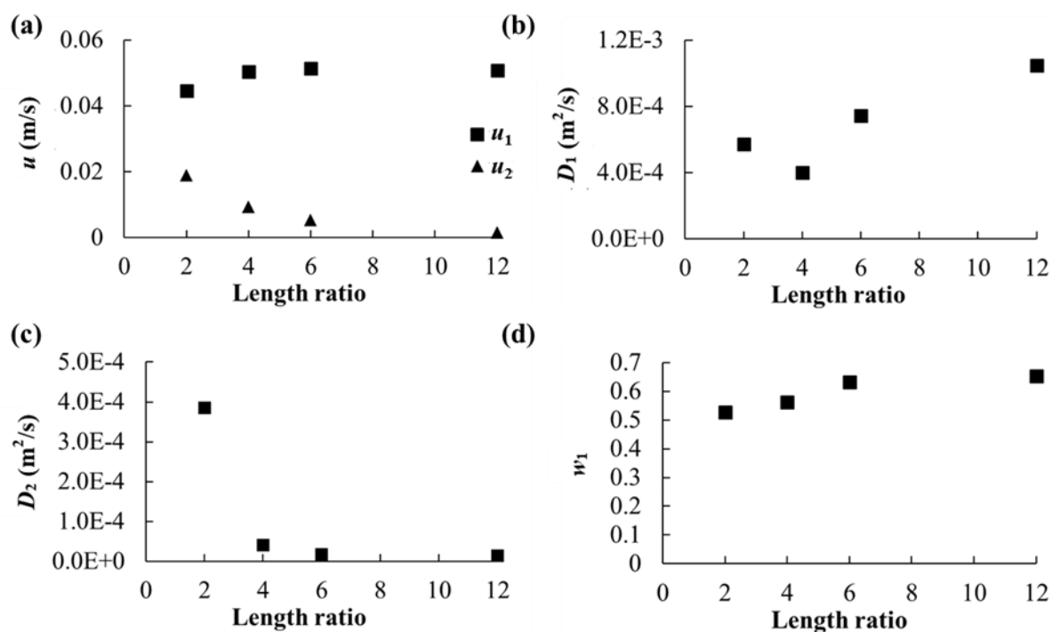
Figure 4. Variation of fitted parameter values with experimental model length for Group 1 experiments. (a) Velocities in the two regions, u_1 and u_2 , (b) Dispersion coefficient of region 1, D_1 , (c) Dispersion coefficient of region 2, D_2 , (d) Water content ratio of region 1, w_1 .
