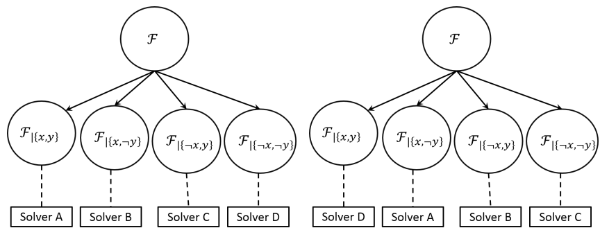
(a) Initially, solvers of the portfolio are regularly distributed over sub-formulas
