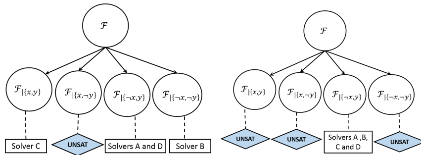
(c) Unsatisfiable sub-formulas are marked in order to prevent other solvers from branching to it again
