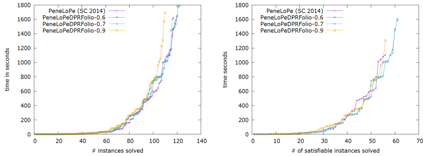
Figure 2 – Cactus plot on the 300 application benchmarks of the SAT Competition 2016: on the left, the cactus plot on all (satisfiable and unsatisfiable) instances. On the right, we have the cactus plot on satisfiable instances only on satisfiable instances where our solvers solve respectively 1 and 5 satisfiable instances more than PENELOPE. Furthermore, we can notice that the main improvement is not the additional number of solved instances but the total run time used to solve these instances. We have for instance, PENELOPEDPRFOLIO-0.6 which solved 27 satisfiable instances in 11,826 seconds while PENELOPE solved 26 instances in 17,639 seconds; so, the time used by PENELOPE to solve 26 instances is far greater than the time needed by PENELOPEDPRFOLIO-0.6 to solve 27 instances. In Fig. 3 we have the cactus plots on the total solved benchmarks and on the total satisfiable solved instances. These plots clearly show that PENELOPEDPRFOLIO outperforms PENELOPE and that the performance is mainly gained on satisfiable instances. This can be explained by the introduction of search space splitting in our approach which helps improve speedup on satisfiable instances.
