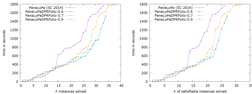
Figure 3 – Cactus plot on the 100 hardest benchmarks of the SAT-Race 2015: on the left, the cactus plot on all (satisfiable and unsatisfiable) instances. On the right, we have the cactus plot on satisfiable instances only
