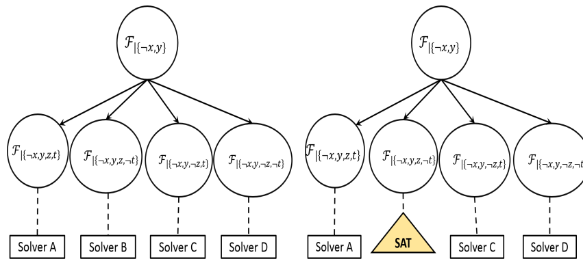
(e) Partitioning (f) The search is stopped if the solver finds a model or if all sub-formulas are unsatisfiable
