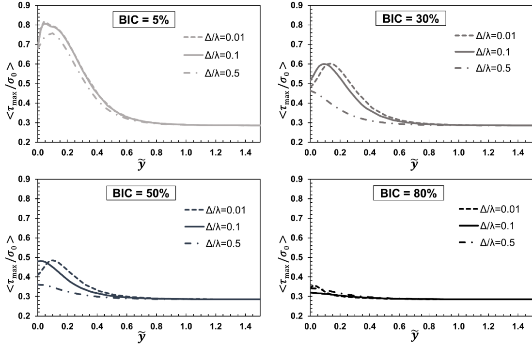
Fig. 5 Variation of the normalized maximal shear stress \tau_{max}/\sigma_0 averaged over x as a function of \tilde{y} . Three values of the waviness ratio \Delta/\lambda = 0.01, 0.1, \text{ and } 0.5 and four values of the BIC ratio equal to 5, 30, 50, 80 % are considered, respectively. Implant and bone Young's moduli are equal to E = 113 \text{ GPa} and E_b = 2 \text{ GPa} , respectively.
