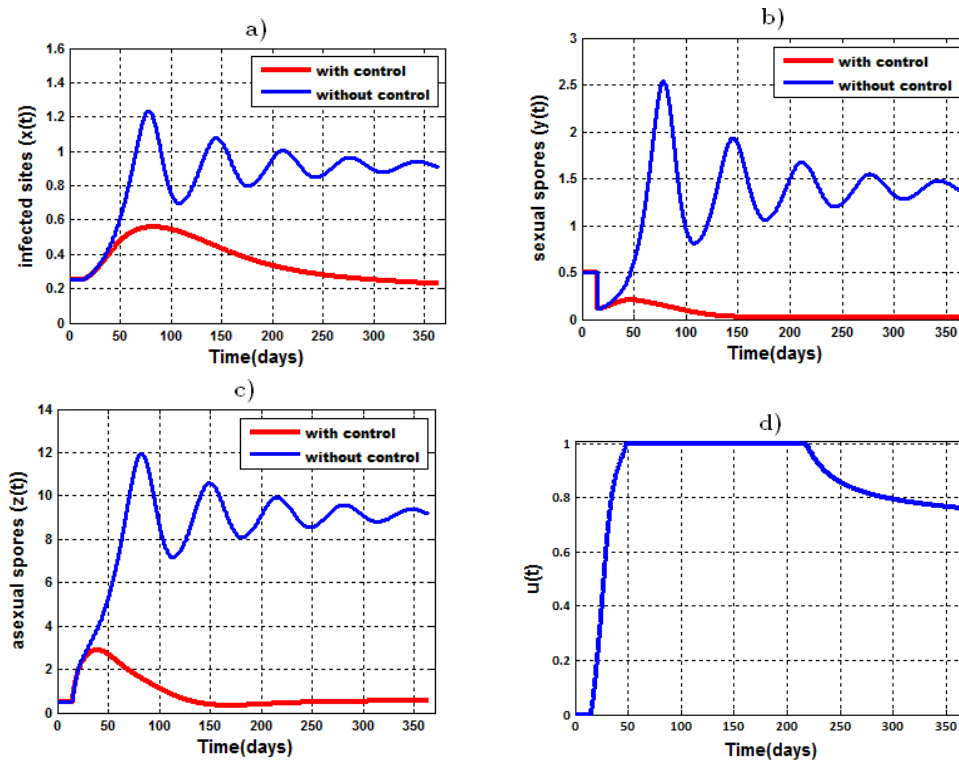
Figure 2: Simulation of system (1) with B = 5 . We can remark that the control is more effective because the weight of infected leaves is high. We can see that the control u(t) (see d)) grows rapidly and reaches its maximum from 50 days and remains so until 230 days( which corresponds to the flowering time [13]) before starting to decrease slowly.
