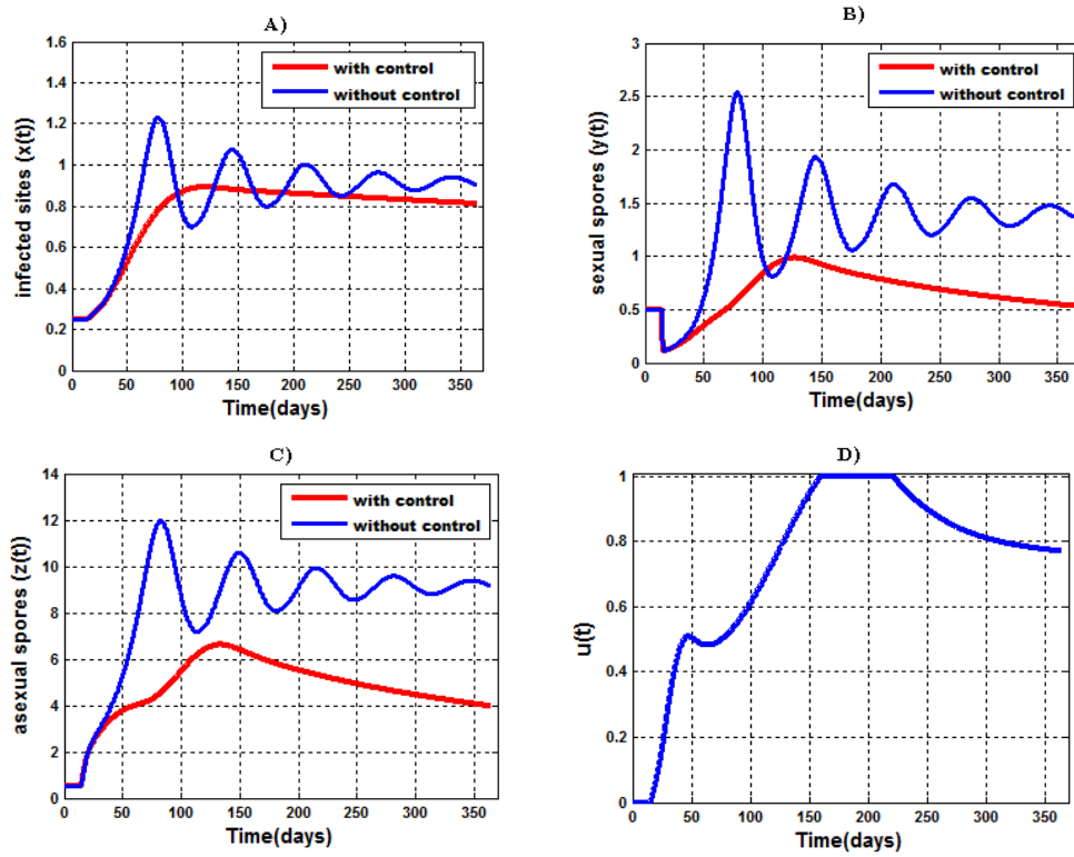
Figure 1: Simulation for B = 2 . We remark that the control is less effective because the weight of control B on the infected leaves is low, nevertheless we can see that the control u(t) (see D)) grows weakly up to 160 days where it reaches its maximum and remains there up to 225 days (which corresponds to the flowering time[13]) and begins to decrease.
