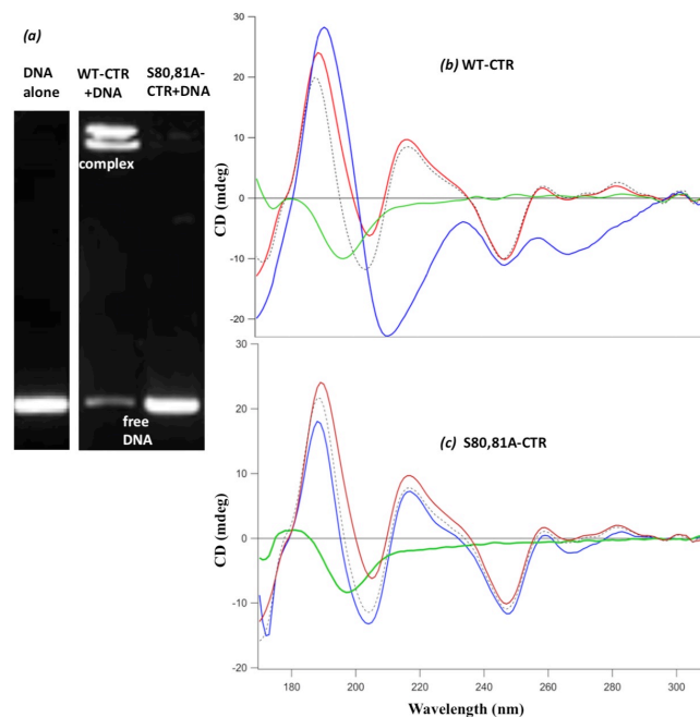
Figure 1: (a) EMSA analysis of Hfq-CTR wild type (WT-CTR) and mutant (S80,81A-CTR) in the presence of DNA. DNA alone; DNA in the presence of WT-CTR; DNA in the presence of S80,81A-CTR mutant. EMSA shows that the mutant does not bind to DNA, while WT-CTR does. Note that 2 complexes of different size are formed by the WT Hfq-CTR, probably due to different numbers of CTRs bound to DNA. (b) SRCD spectra of the WT-CTR/DNA complex (blue), DNA (red) and WT-CTR (green). The dotted spectrum represents the relevant combination of the spectra pertaining to the individual components. (c) As in panel (b) but for S80,81A-CTR.
