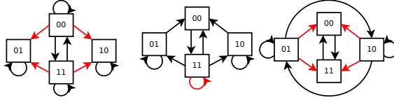
Fig. 5: States transitions diagrams corresponding to three semantics that do not respect Theorem 2 (in black) applied on the Boolean network of Figure 4. Using the synchronous semantics on the optimal program of the black transitions will produce in addition the red ones.
