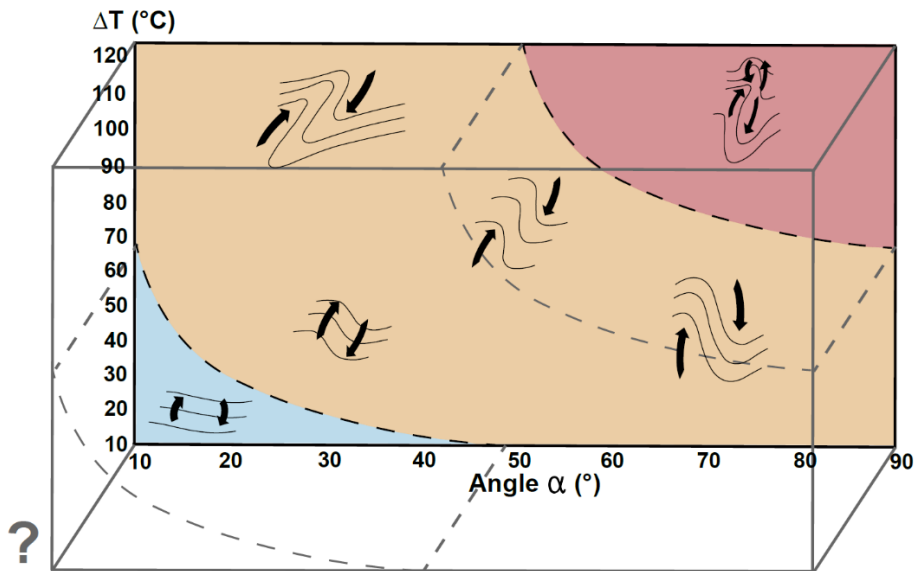
Figure 8 : Diagram of 2D convective regimes for the theoretical fault. Black curves represent isotherm morphology. The dashed black line separate three area. In blue, the area of unicellular weak type convection zone. In orange the area of unicellular medium type convection zone. In red, the area of bicellular strong type convection zone. The third variable, which may be used for 3D experiments has yet to be determined.
