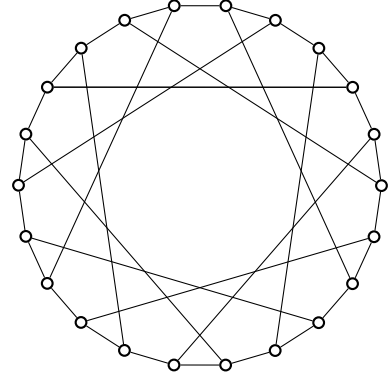
(c) A bipartite graph with \omega^{[\#2]}(G) = 4 and \chi^{[\#2]}(G) = 6
