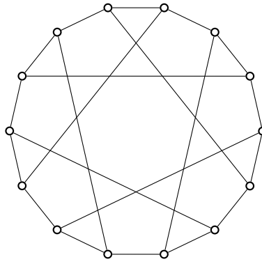
(b) The Heawood graph : \omega^{[\#2]}(G) = \chi^{[\#2]}(G) = 7
