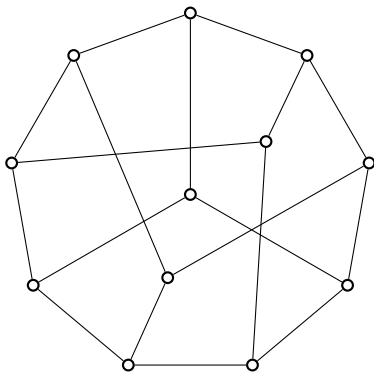
(a) The triplex graph with \omega^{[\#2]}(G) = \chi^{[\#2]}(G) = 6
