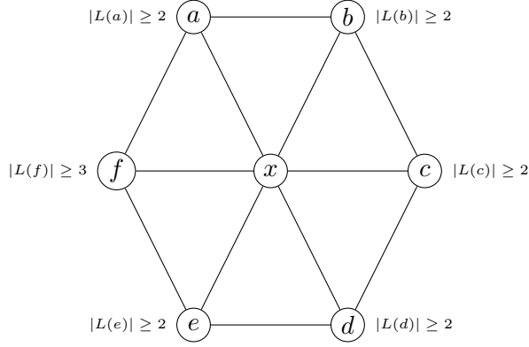
Figure 9: Graph of Lemma 22, where L(x) = \{1, 2, 3, 4, 5\} .
