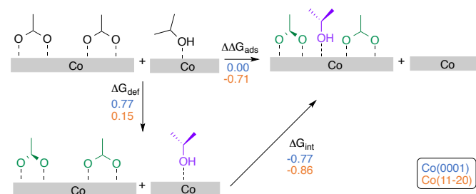
Scheme 1. Decomposition of the variation of Gibbs Free energy of adsorption of iPrOH on Co induced by the presence of acetate ligands ( \Delta\Delta G_{ads} ) into deformation ( \Delta G_{def} ) and interaction ( \Delta G_{int} ). The corresponding values are reported in eV for the Co(0001) and Co(11-20) surfaces in blue and orange, respectively. Details are reported in supplementary information (Table S4).
