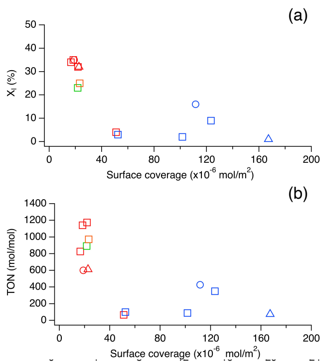
Figure 3. (a) 2-octanol conversion (X i , %) and (b) turn-over number (TON, mol mol -1 ) as a function of the surface coverage. The points correspond to the Co nanoparticles (Table 1, Table 2): nanorods (□), diabolos (△), platelets (○). The color of the symbols represents (the type of decorating ligand: palmitate (blue), laurate (red), decanoate (orange), octanoate (green)).
