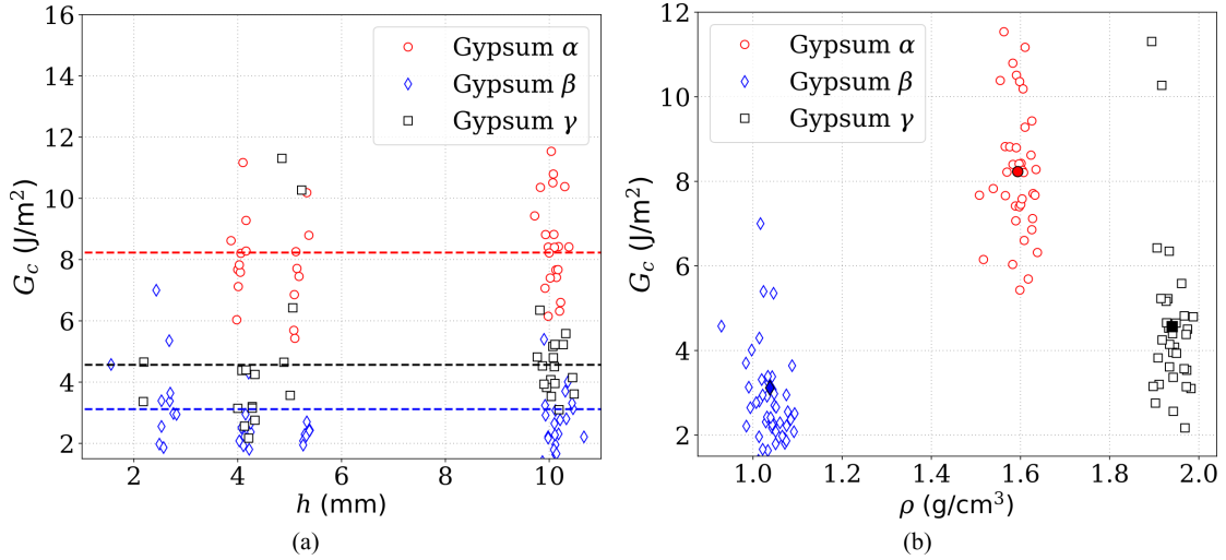
Figure 9: Fracture toughness \mathcal{G}_c identified from experimental measurements of specimen height h and maximum flexural stress \sigma_{\max} on gypsum specimens assuming \sigma_c = 9.5 \text{ J/m}^2 ( \alpha -gypsum), \sigma_c = 2.7 \text{ J/m}^2 ( \beta -gypsum) and \sigma_c = 12 \text{ J/m}^2 ( \gamma -gypsum) as a function of specimen a) height h and b) density \rho .
