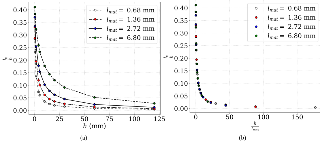
Figure 6: Initiation crack length to specimen height ratio for several ( \mathcal{G}_c , \sigma_c ) couples corresponding to different material characteristic lengths l_{mat} as a function of a) the specimen size and b) specimen height to material characteristic length ratio.
