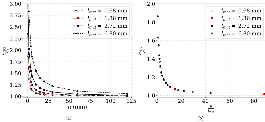
Figure 7: Maximum flexural stress to strength ratio for several ( \mathcal{G}_c , \sigma_c ) couples corresponding to different material characteristic lengths l_{mat} as a function of a) the specimen size and b) specimen height to material characteristic length ratio.
